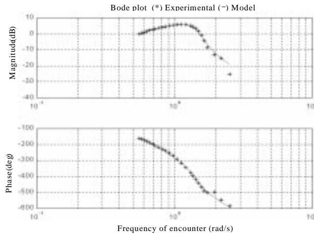
Figure 4: Bode plot of G_P(s) and data of PRECAL program
